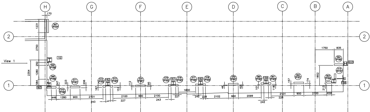
MAGISTRATES COURT PLAN, FIFTH FLOOR (REFER DRG 021 FOR BUILDERS DETAILS)
